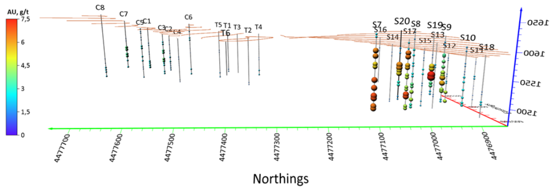
Figure 3 – Initial 3D visualization of component concentration along borehole depth (UTM Zone 38 coordinate system in meters)
